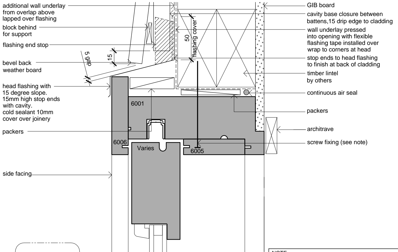
Door Head Scale: 1:2.5
