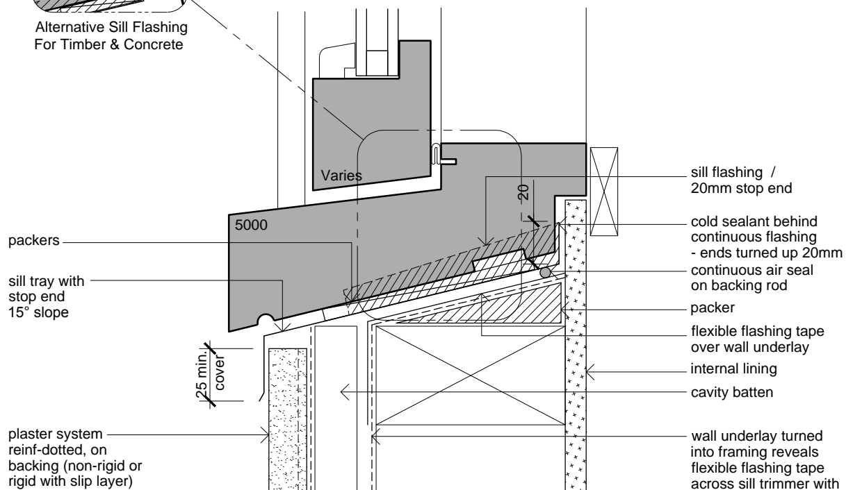
Window Sill
