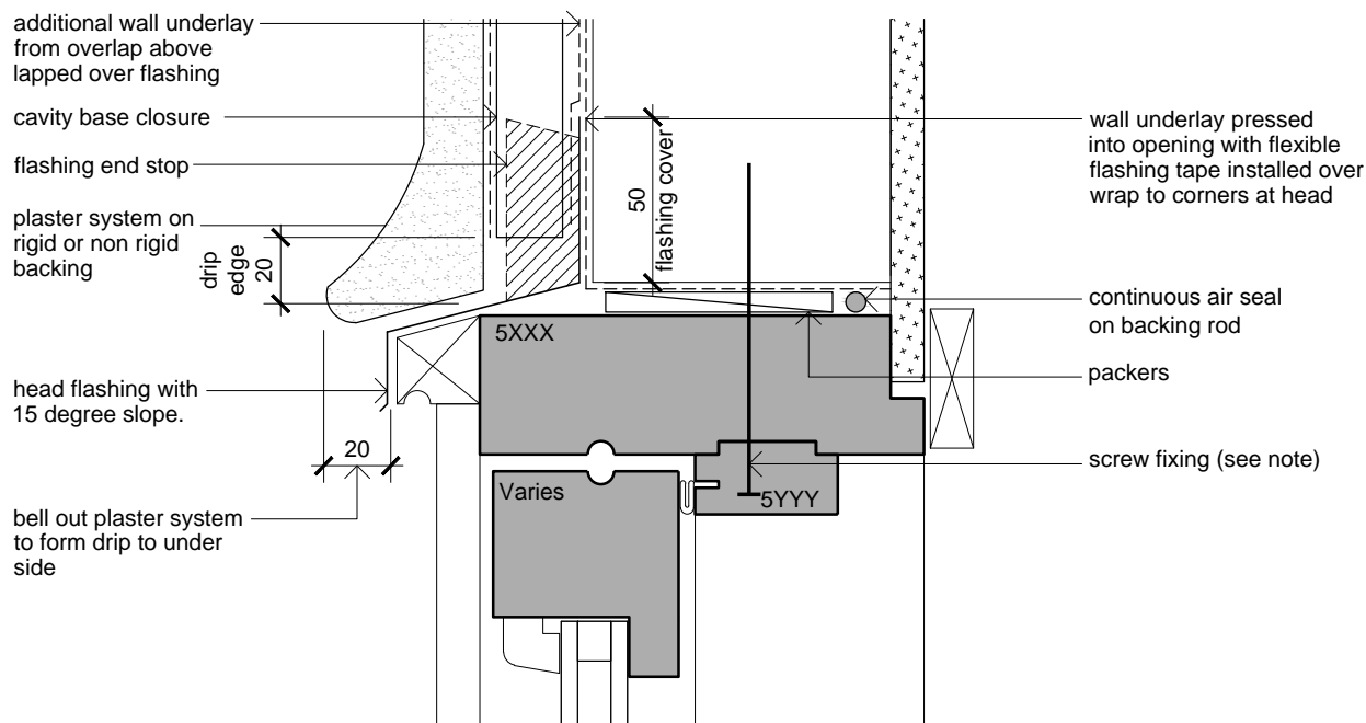
Window Head
