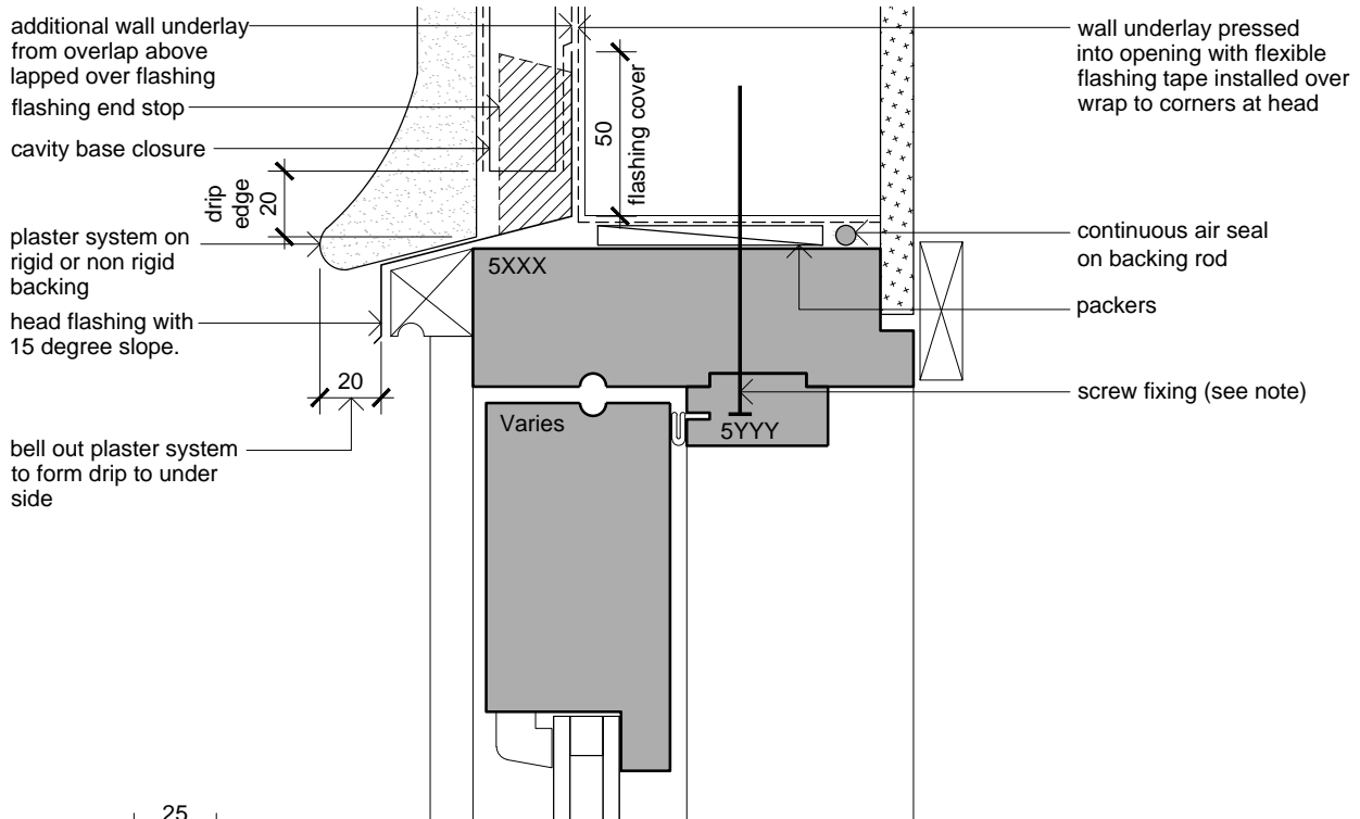
Door Head Scale: 1:2.5
