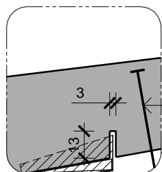
Alternative Sill Flashing For Timber & Concrete
