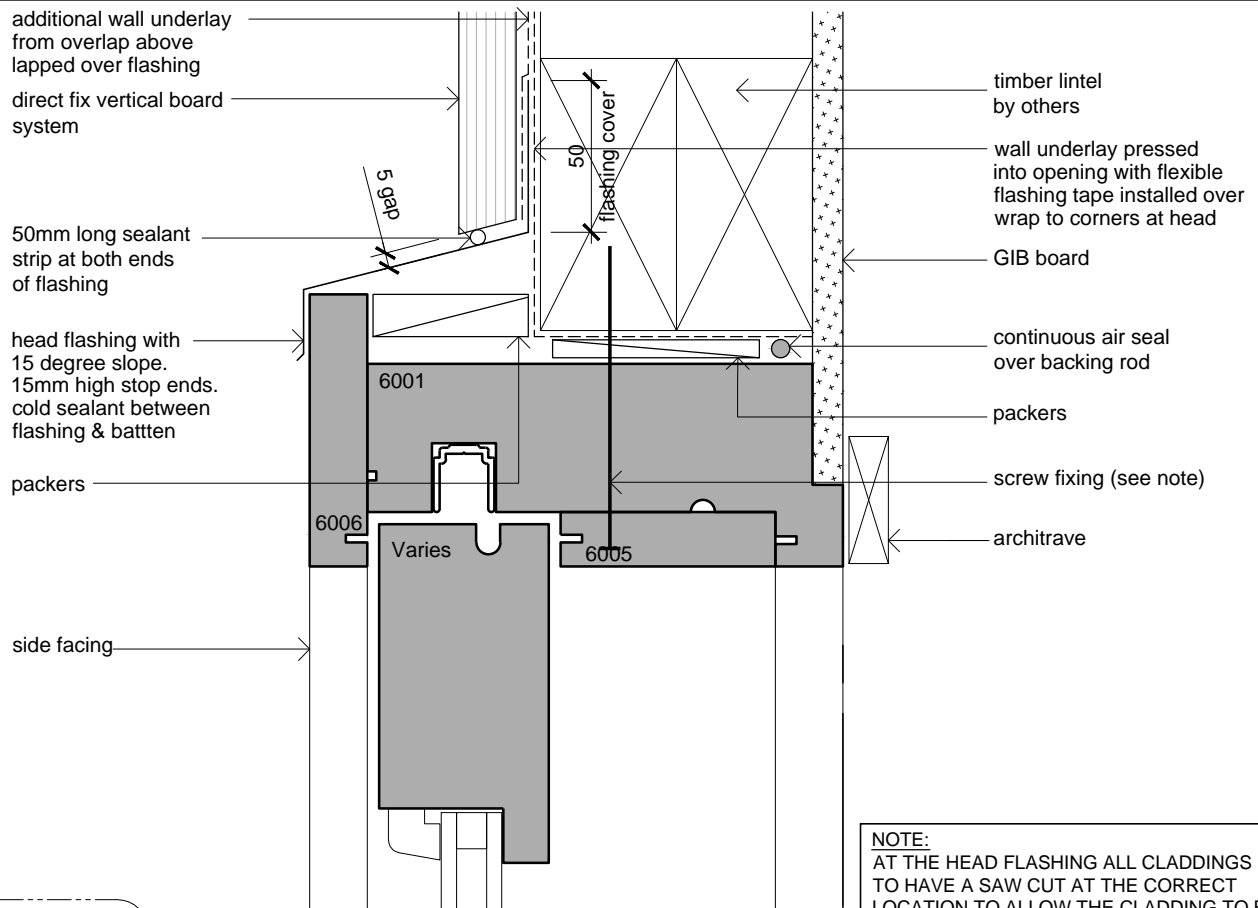
Door Head Scale: 1:2.5
