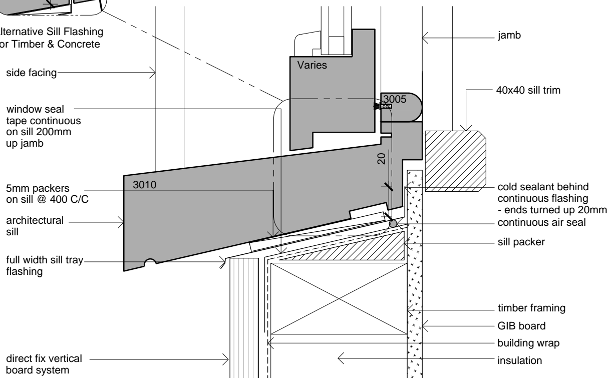
Window Sill
