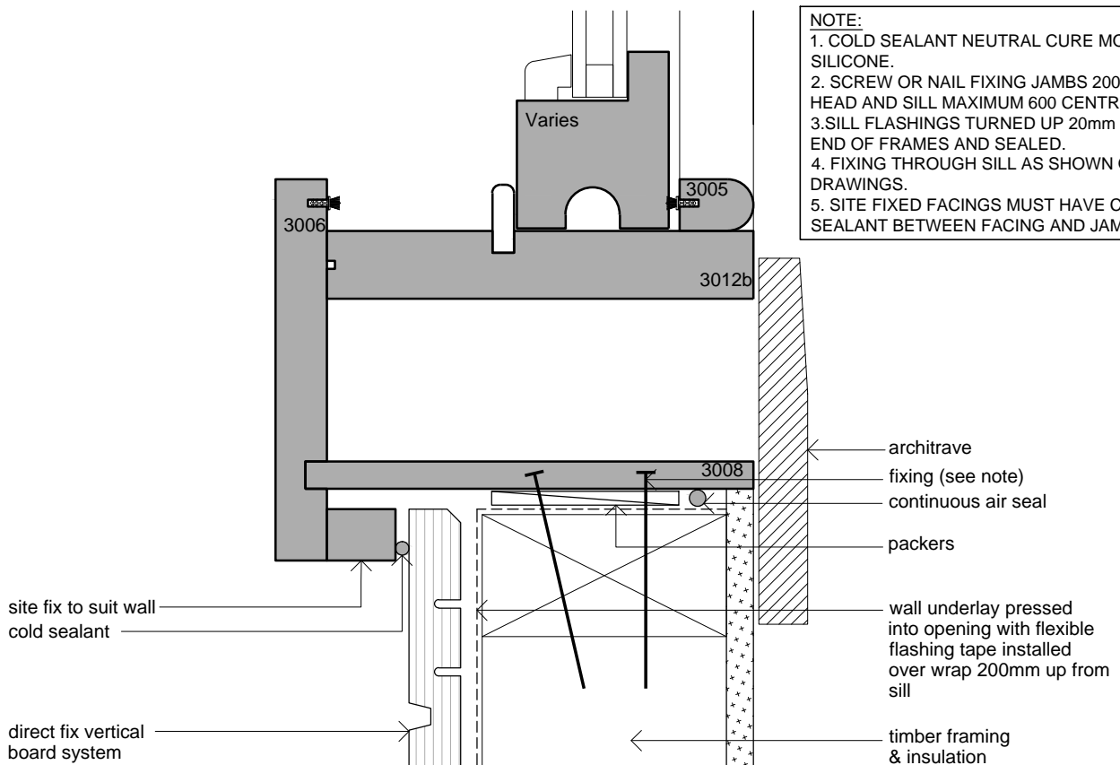
Window Jamb (Lower)
