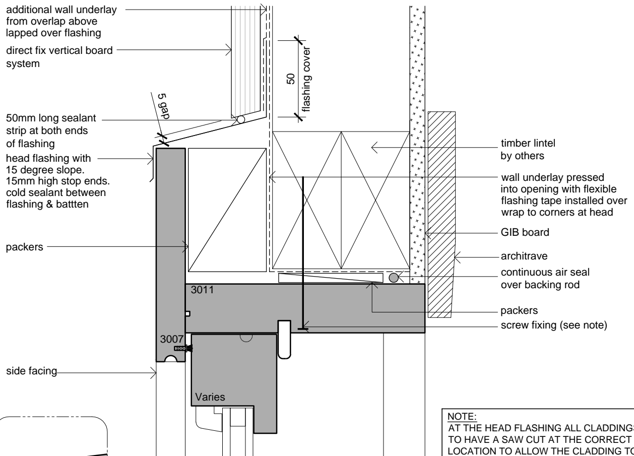
Window Head
