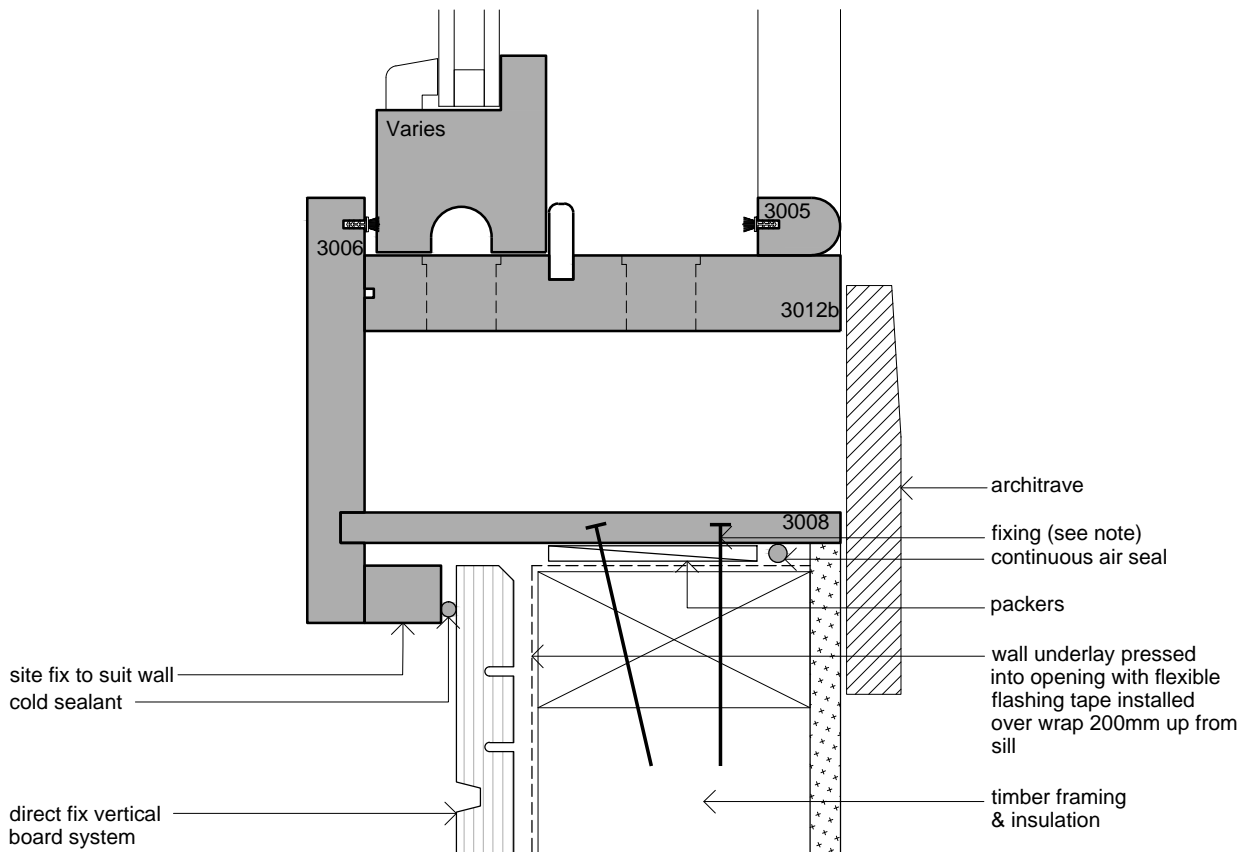
Window Jamb (Upper)
