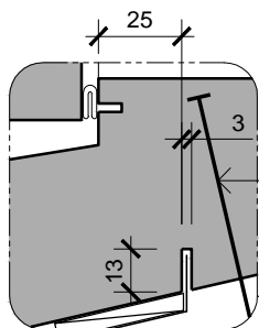
Alternative Sill Flashing For Timber & Concrete
