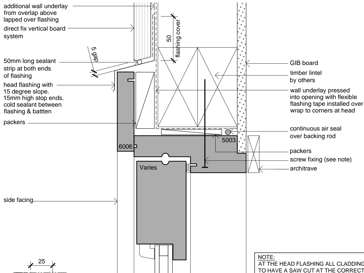
Door Head Scale: 1:2.5
