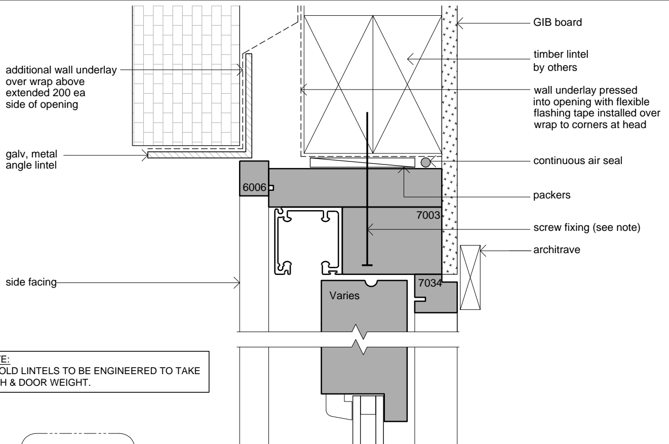
Door Head Scale: 1:2.5
