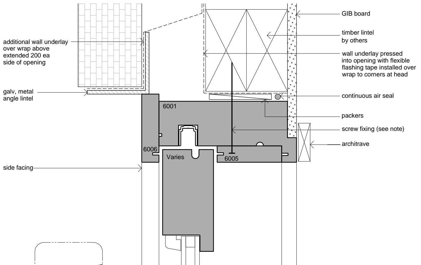
Door Head Scale: 1:2.5
