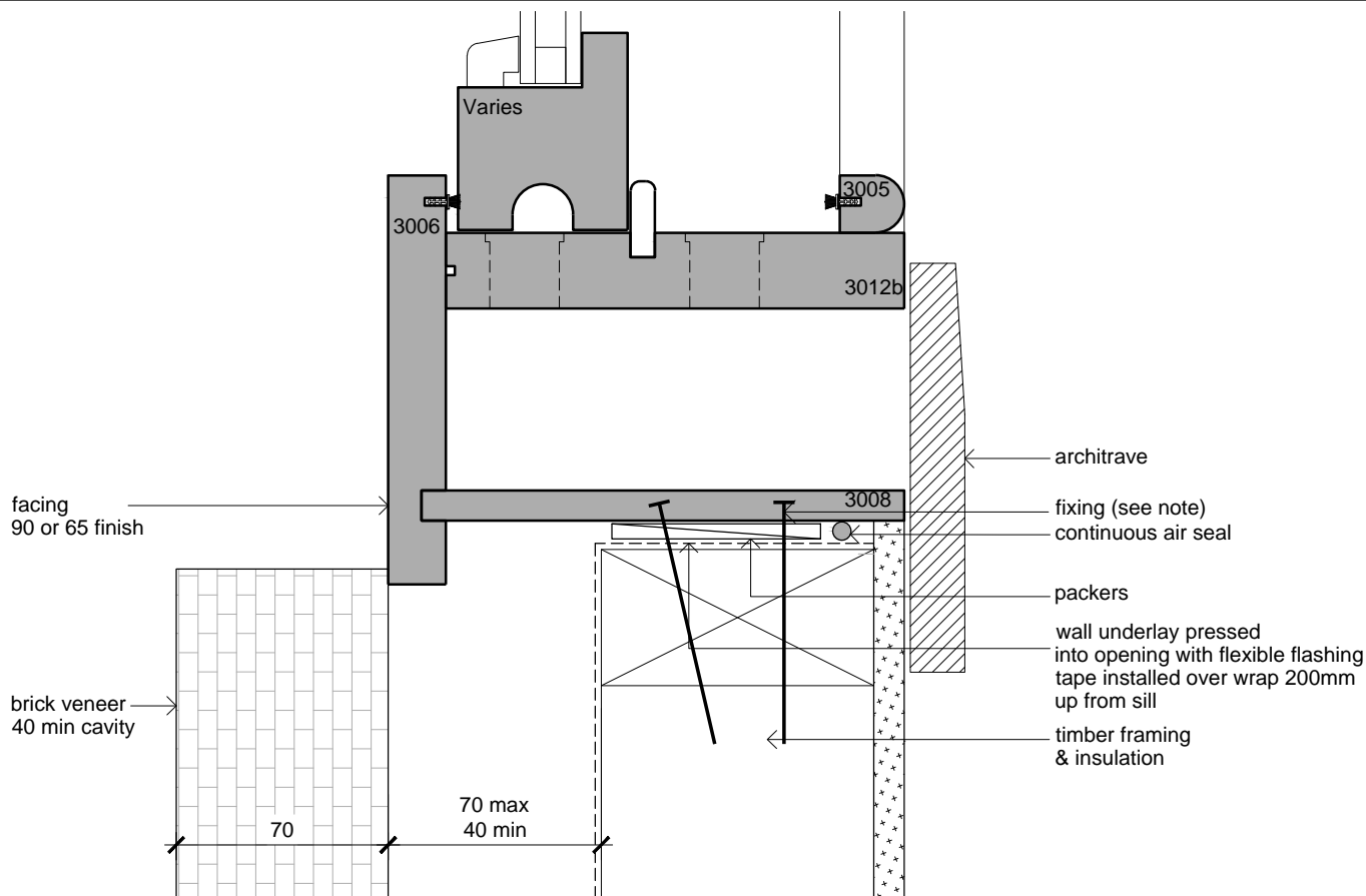
Window Jamb (Upper)
