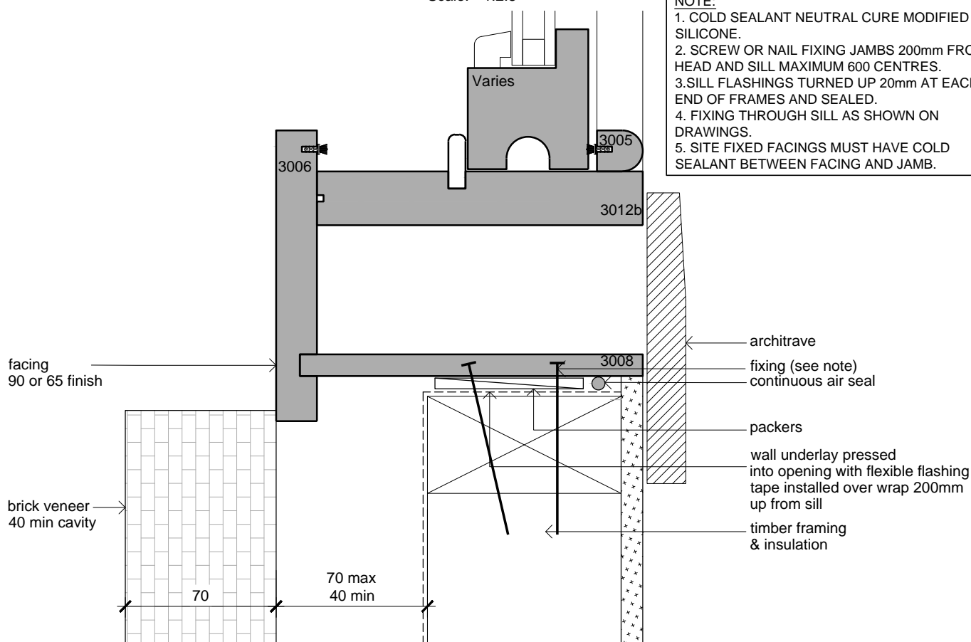
Window Jamb (Lower)
